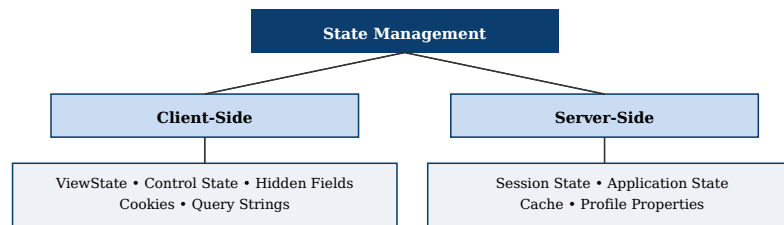
Fig 21.1: Classification of ASP.NET state management techniques
