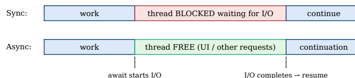
Fig 16.1: await frees the thread during I/O instead of blocking it
