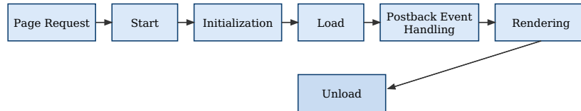
Fig 7.1: Stages of the ASP.NET Web Forms page life cycle
